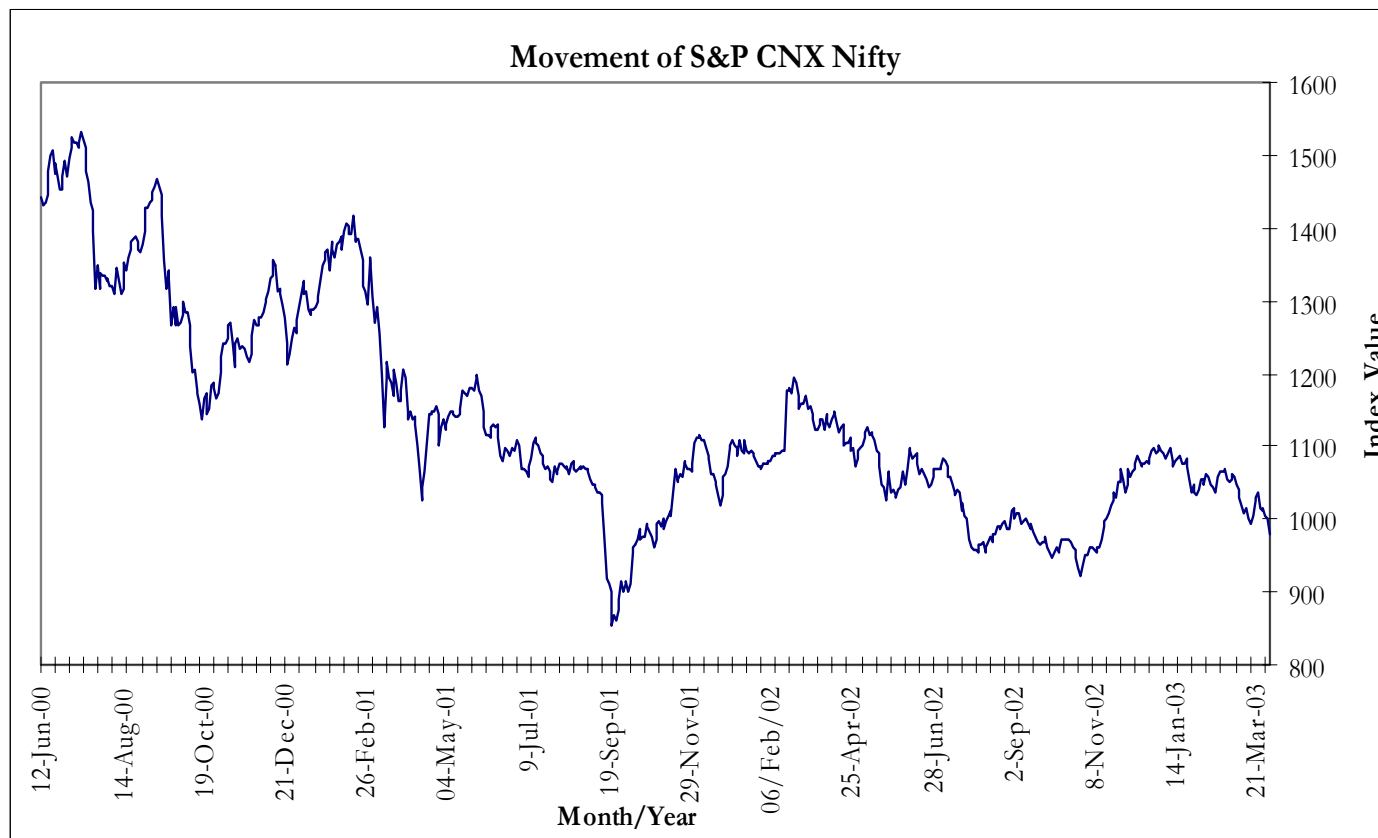
Chart 5.1: Movement of S&P CNX Nifty
