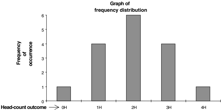
Frequency Distribution
