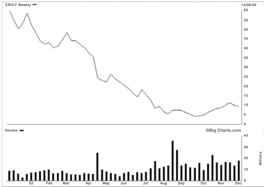
Figure 11-4 Downtrend
